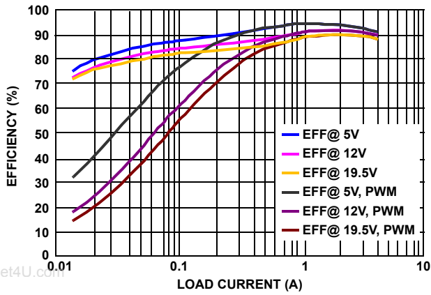
FIGURE 1. EFFICIENCY OF CHANNEL 1, 2.5V, HYS/PWM MODE
