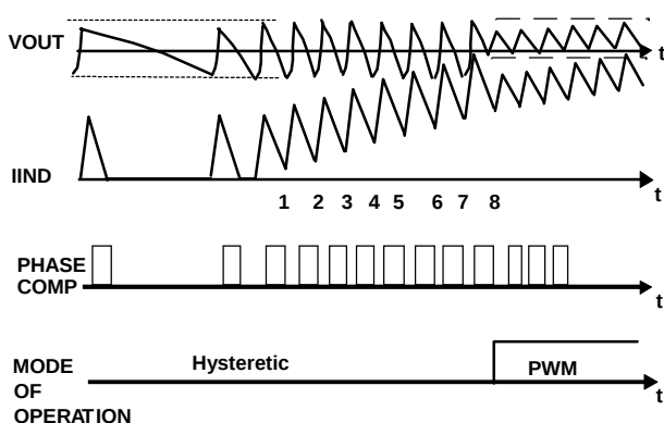
FIGURE 36. HYSTERETIC—CCM TRANSITION
