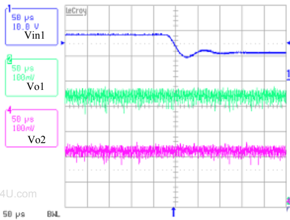
FIGURE 13. INPUT STEP-DOWN TRANSIENT AT PWM MODE
