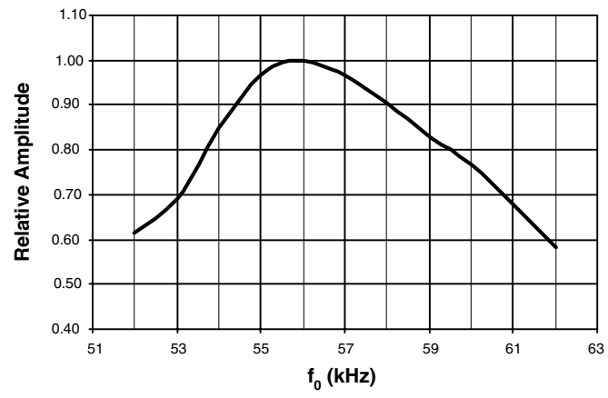
Figure 9. Typical Bandpass Curve at T_{\text{amb}} = 25^{\circ}\text{C}
