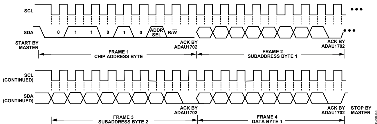
Figure 20. I²C Write to ADAU1702 Clocking
