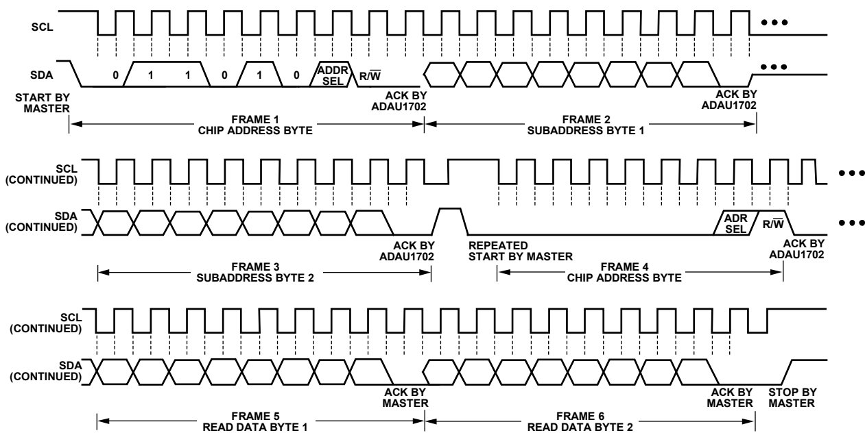
Figure 21. I²C Read from ADAU1702 Clocking
