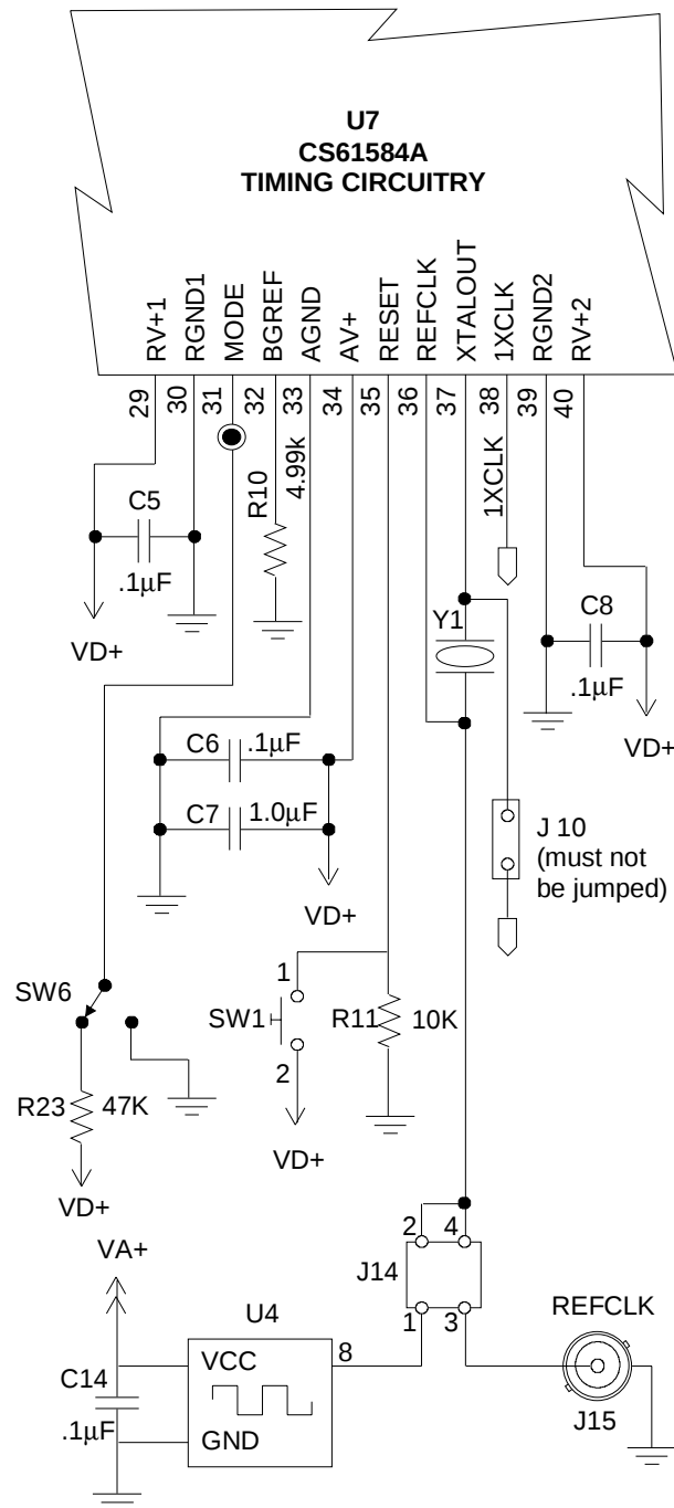
Figure 4. Timing Circuitry
