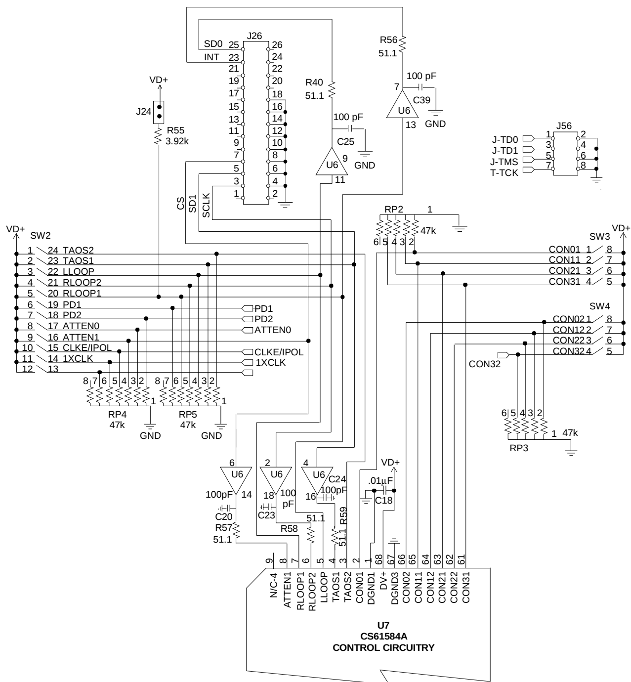
Figure 3. Control Circuitry
