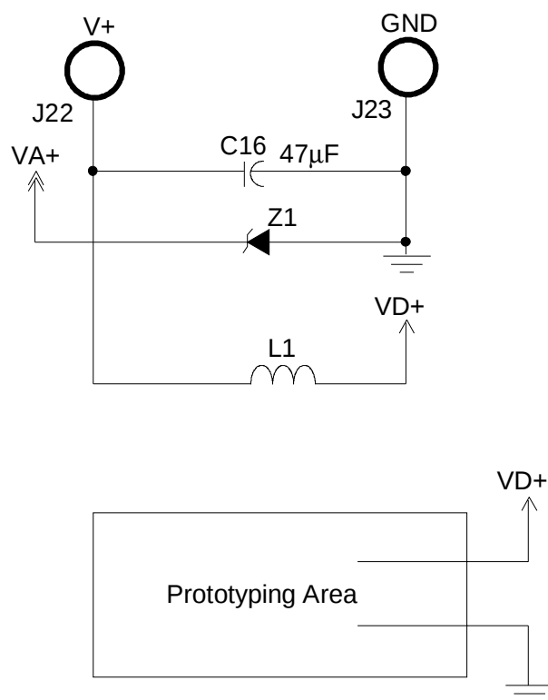
Figure 5. Common Circuitry
