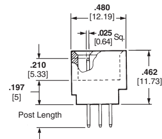
Solder Posts
