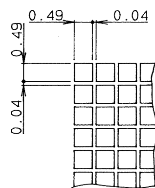
DOT DETAIL Scale 10/1
