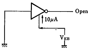
Test Circuit 3 ( V_{EB} )
