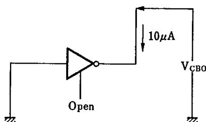
Test Circuit 1 ( V_{CB0} )
