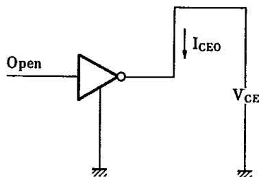
Test Circuit 4 ( I_{CE0} )
