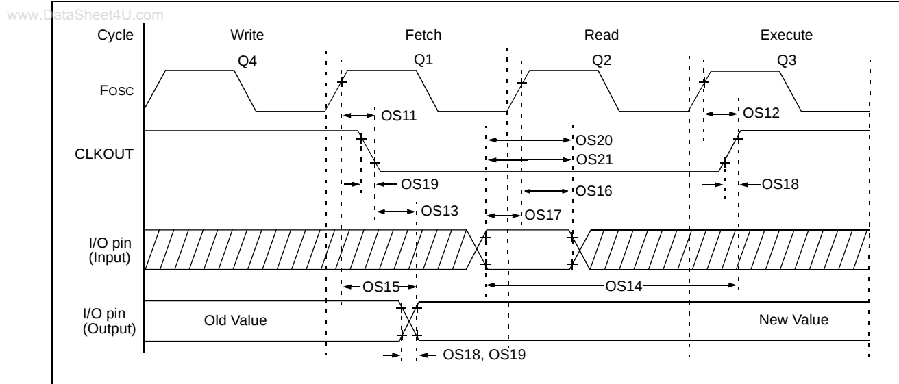
FIGURE 17-5: CLKOUT AND I/O TIMING
