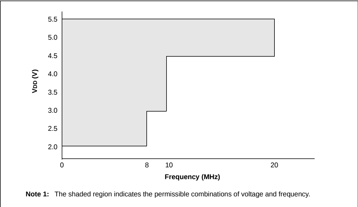
FIGURE 17-1: PIC16F882/883/884/886/887 VOLTAGE-FREQUENCY GRAPH, -40°C ≤ TA ≤ +125°C
