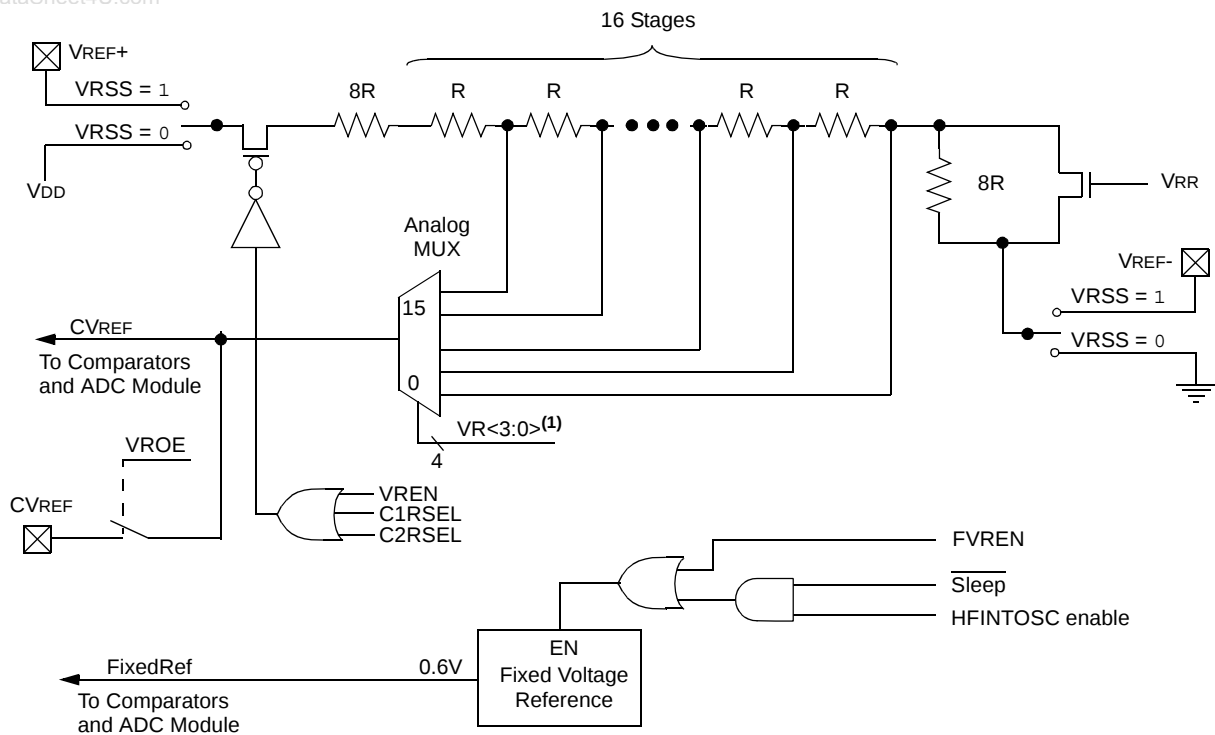
FIGURE 8-8: COMPARATOR VOLTAGE REFERENCE BLOCK DIAGRAM
