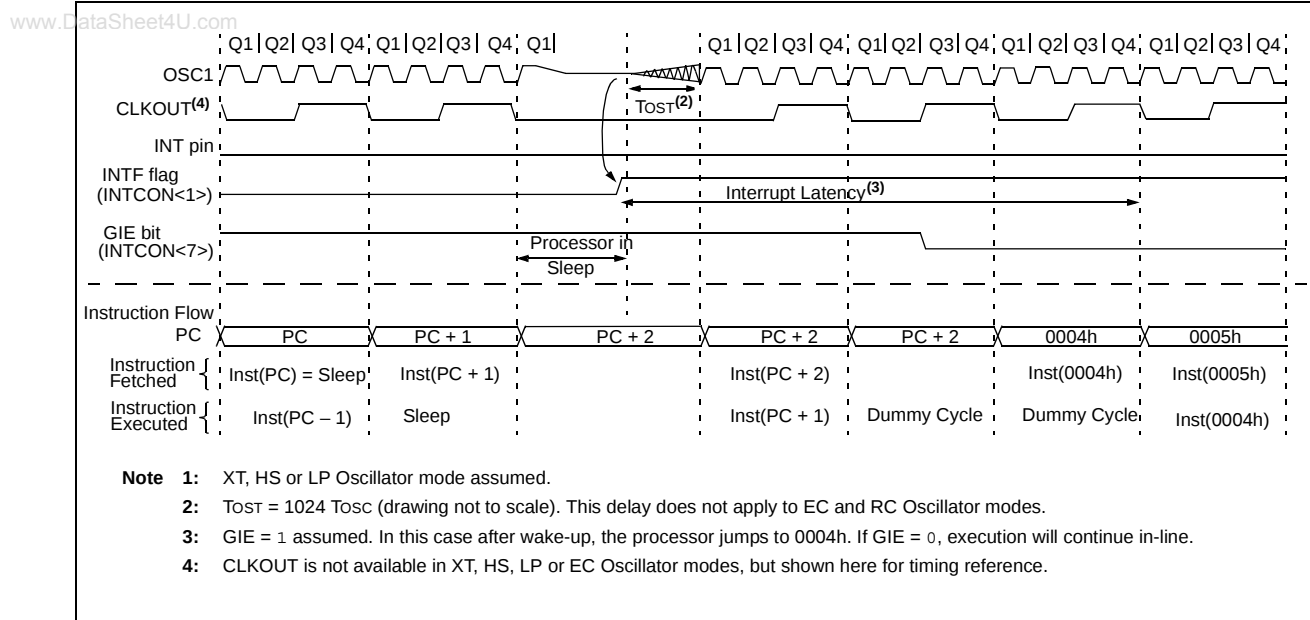
FIGURE 14-10: WAKE-UP FROM SLEEP THROUGH INTERRUPT
