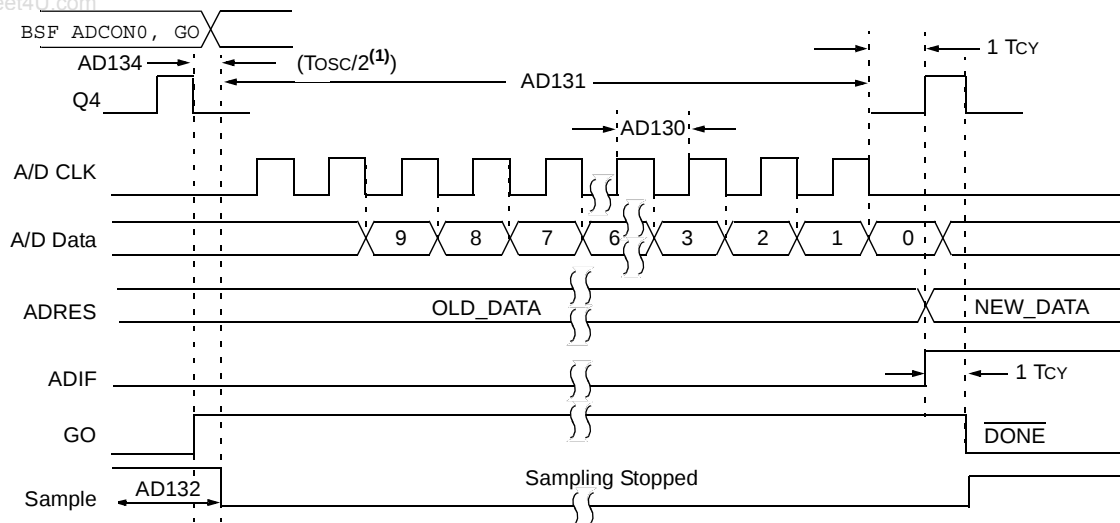
FIGURE 17-10: PIC16F882/883/884/886/887 A/D CONVERSION TIMING (NORMAL MODE)
