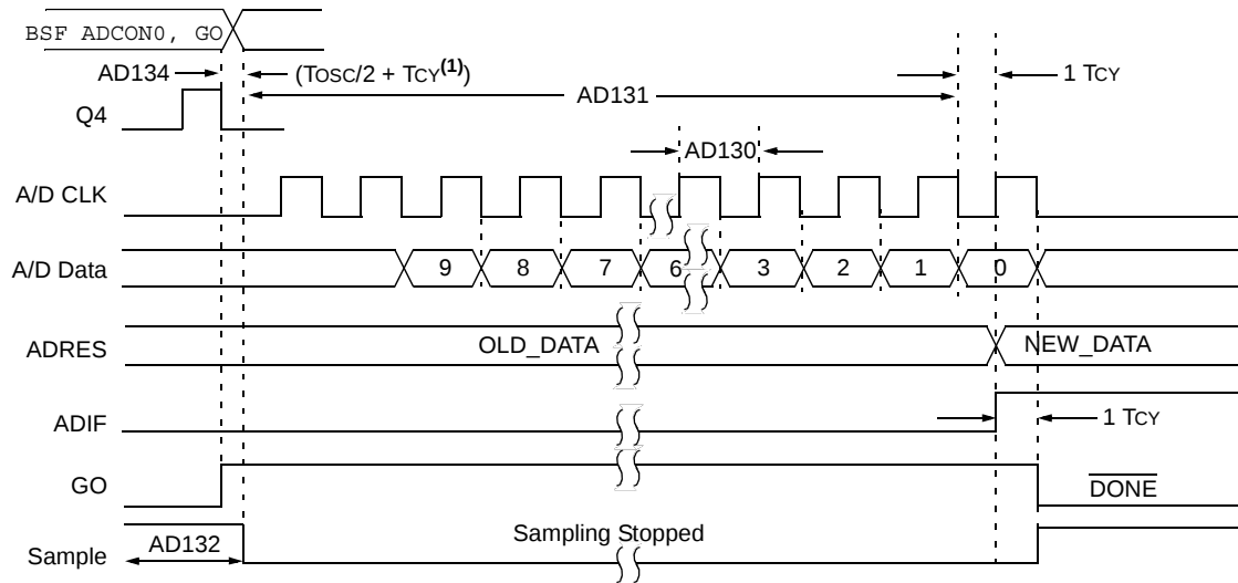
FIGURE 17-11: PIC16F882/883/884/886/887 A/D CONVERSION TIMING (SLEEP MODE)
