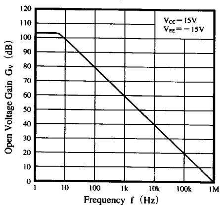
G_V - f
