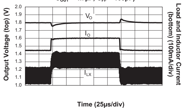
Load Transient Response (350mA to 500mA; V_{IN} = 3.6V ; V_{OUT} = 1.8V ; C_{OUT} = 4.7\mu F ; C_{FF} = 100pF )
