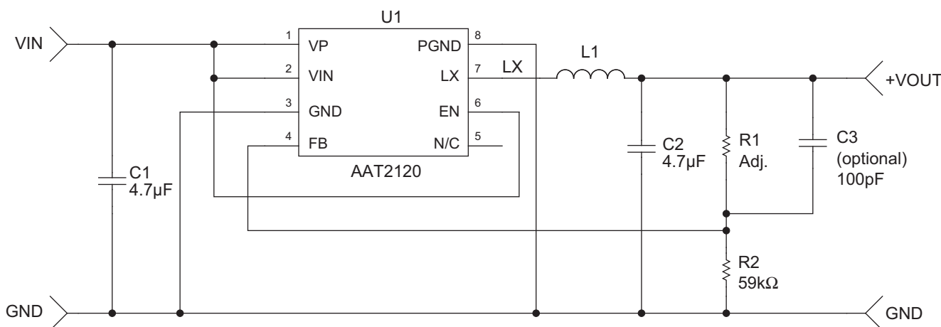
Figure 1: AAT2120 Schematic.
