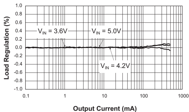
Load Regulation (V_{OUT} = 3.0V; L = 4.7\mu H)
