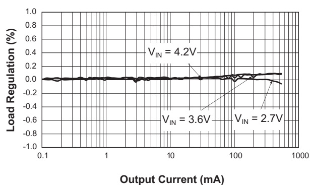
Load Regulation (V_{OUT} = 1.8V; L = 3.3\mu H)
