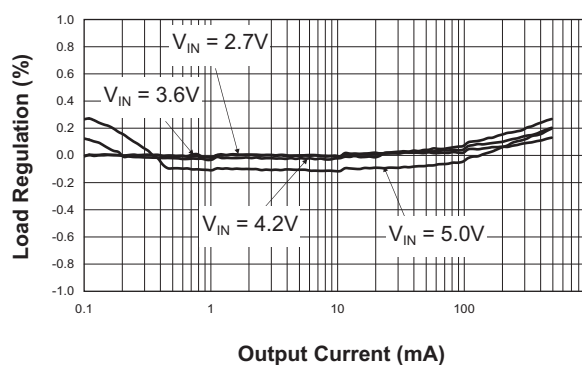
Load Regulation (V_{OUT} = 1.2V; L = 1.5\mu H)
