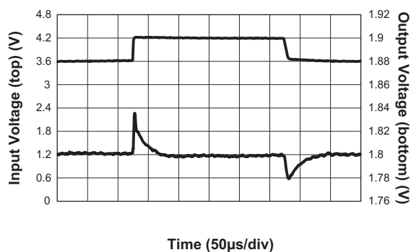
Line Transient
