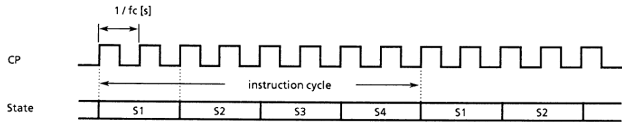
Figure 2-17. Instruction Cycle
