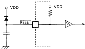
Figure 2-23. Simplified Power-On-Reset
