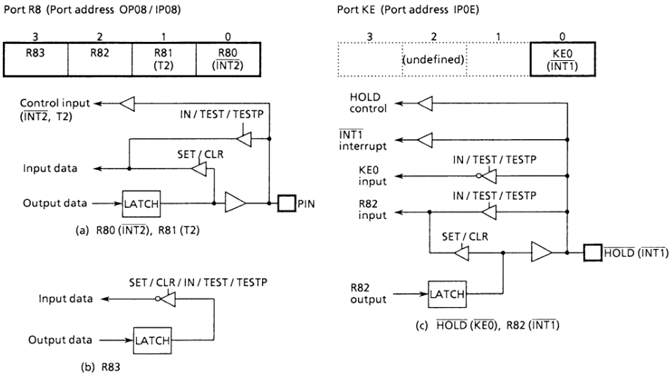
Figure 3-4. Port R8 and HOLD (INT1) Pin
