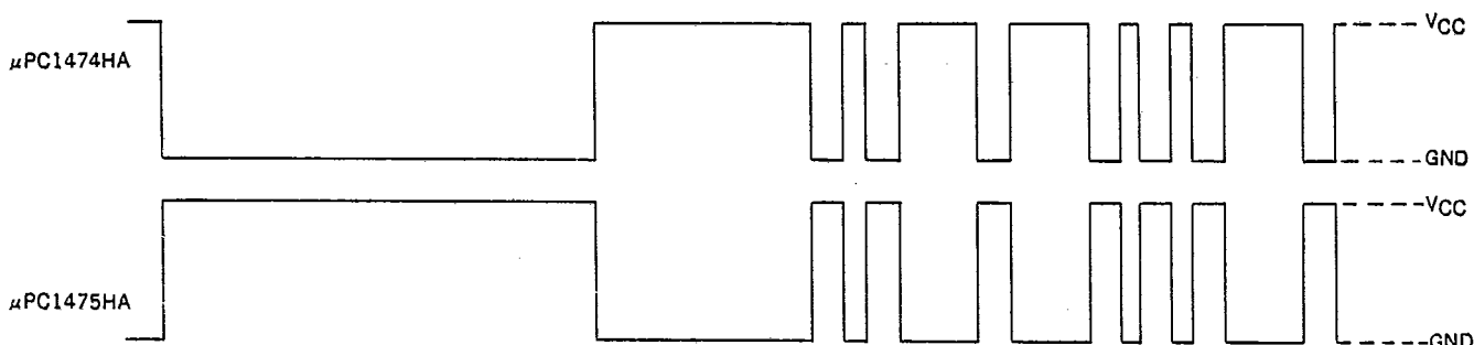
Output Waveform
