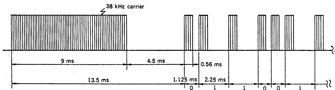
Output Waveform
