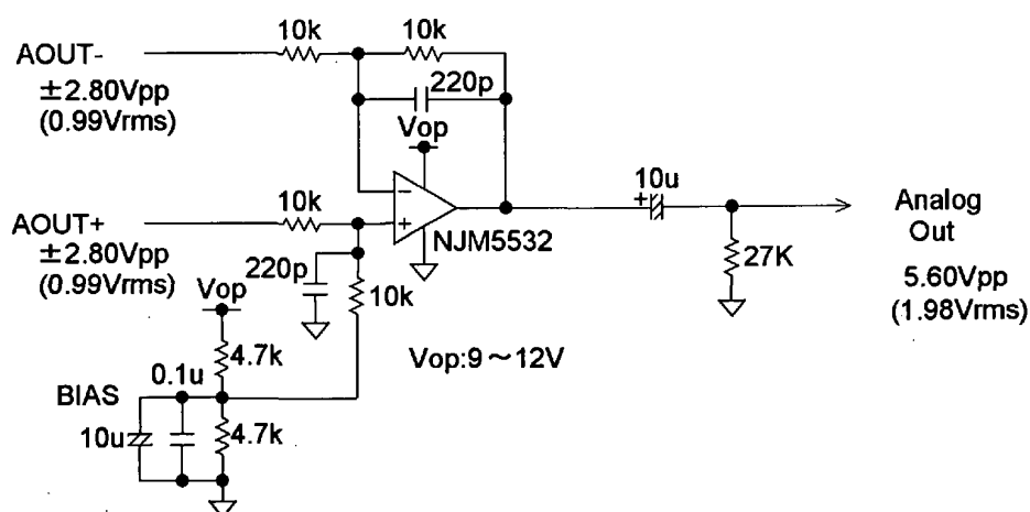
Figure 9 . External LPF example
