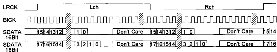
Figure 4 . Mode 2 Timing
