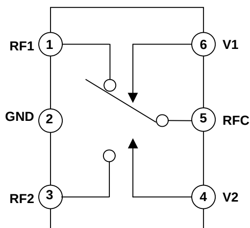
Function Block Diagram
