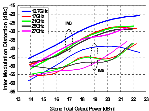
IMD vs. Output Power @ VDD=6V, IDD(DC)=300mA
