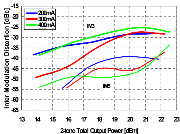
IMD vs. Output Power by Drain Current @f=17GHz, VDD=6V
