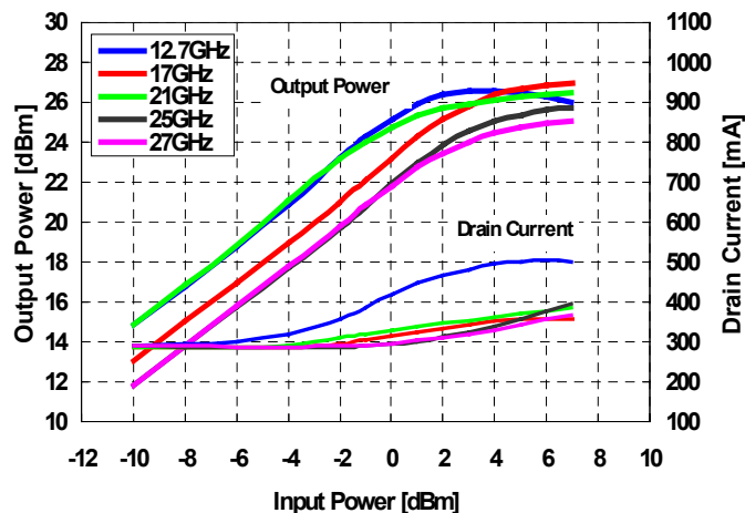
Output Power, Drain Current vs. Input Power @ VDD=6V, IDD(DC)=300mA
