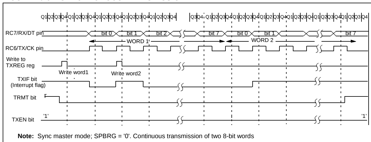
FIGURE 10-9: SYNCHRONOUS TRANSMISSION
