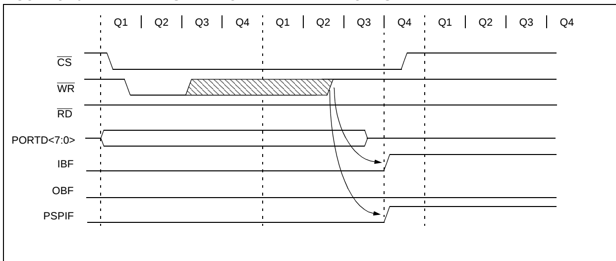
FIGURE 3-10: PARALLEL SLAVE PORT WRITE WAVEFORMS
