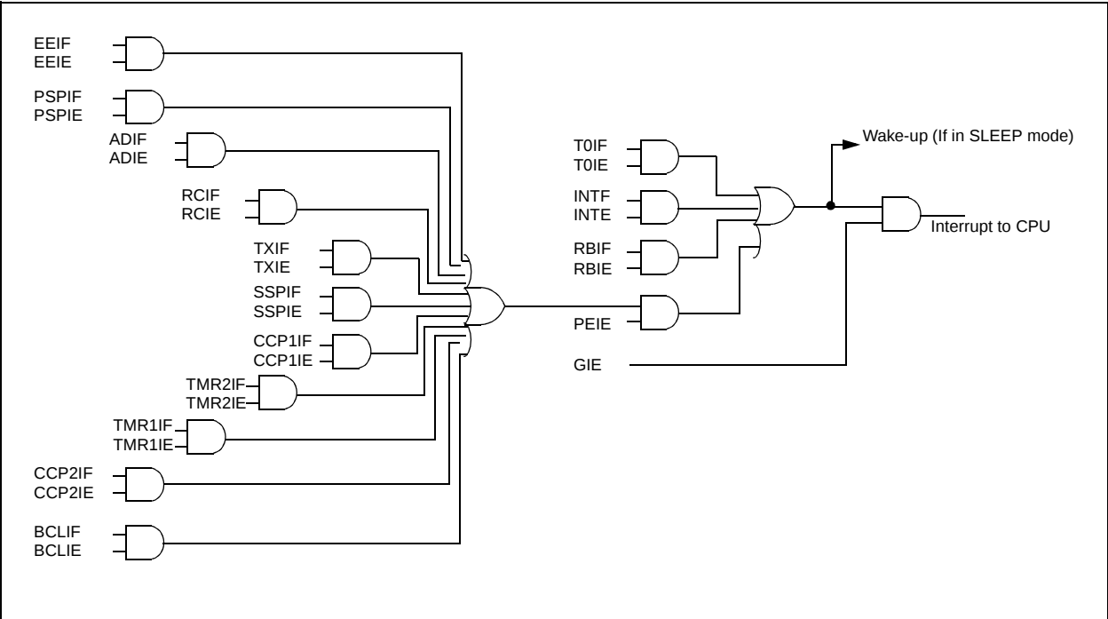
FIGURE 12-9: INTERRUPT LOGIC
