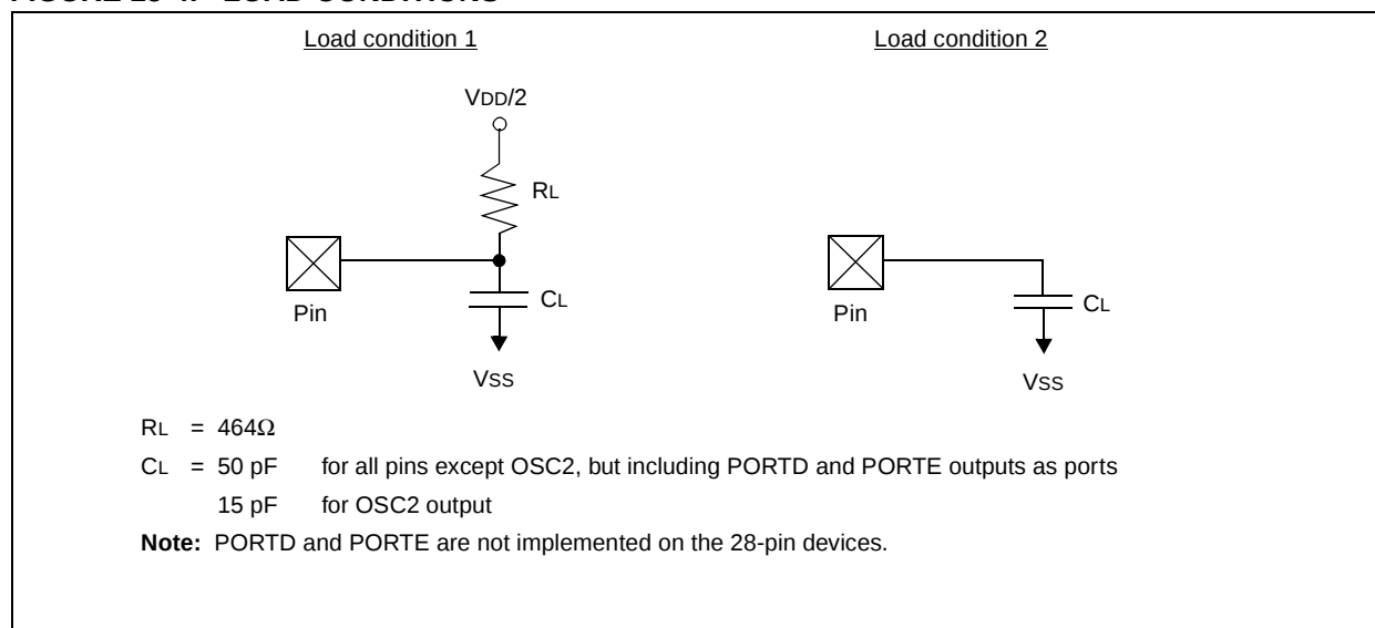
FIGURE 15-4: LOAD CONDITIONS
