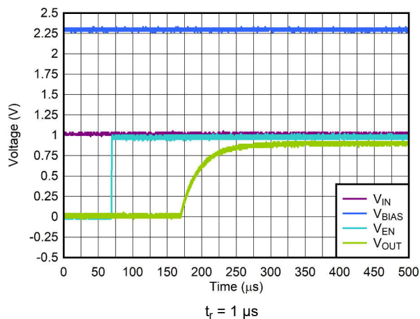
Figure 6-15. Start-Up With V_{\text{IN}} and V_{\text{BIAS}} Before V_{\text{EN}}
