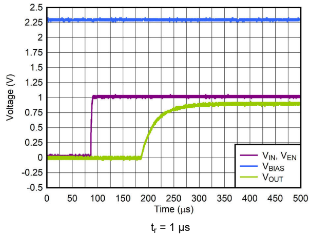
Figure 6-13. Start-Up With V_{\text{BIAS}} Before V_{\text{IN}}
