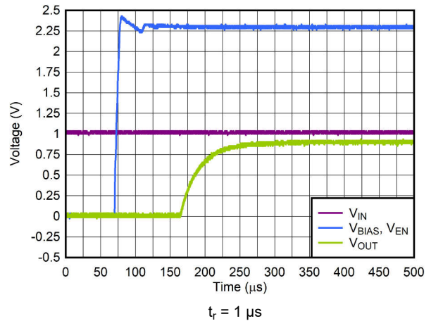
Figure 6-14. Start-Up With V_{\text{IN}} Before V_{\text{BIAS}} and V_{\text{EN}}
