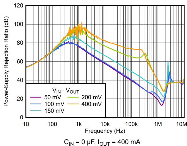
Figure 6-21. V_{\text{IN}} PSRR vs Frequency and V_{\text{IN}} - V_{\text{OUT}}
