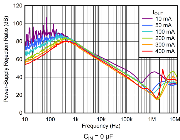
Figure 6-23. V_{\text{IN}} PSRR vs Frequency and I_{\text{OUT}}
