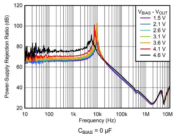
Figure 6-24. V_{\text{BIAS}} PSRR vs Frequency and V_{\text{BIAS}} - V_{\text{OUT}}
