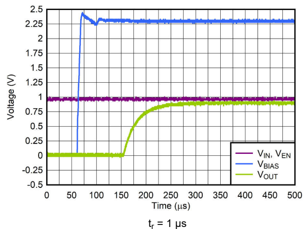
Figure 6-16. Start-Up With V_{\text{IN}} and V_{\text{EN}} Before V_{\text{BIAS}}
