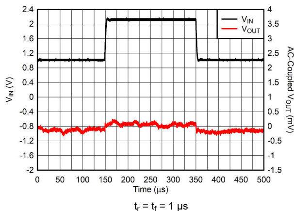
Figure 6-17. Line Transient From 1 V to 2.2 V
