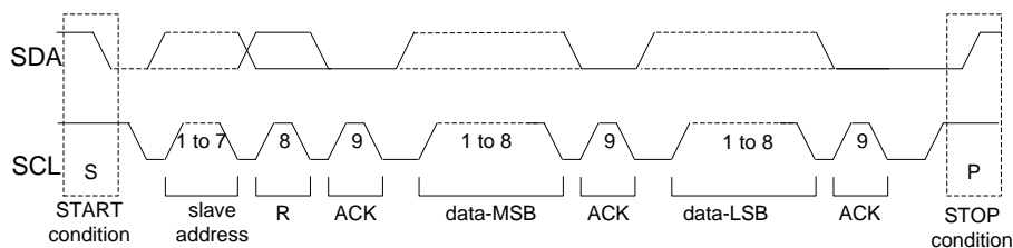
Figure 36. Read Sequence
