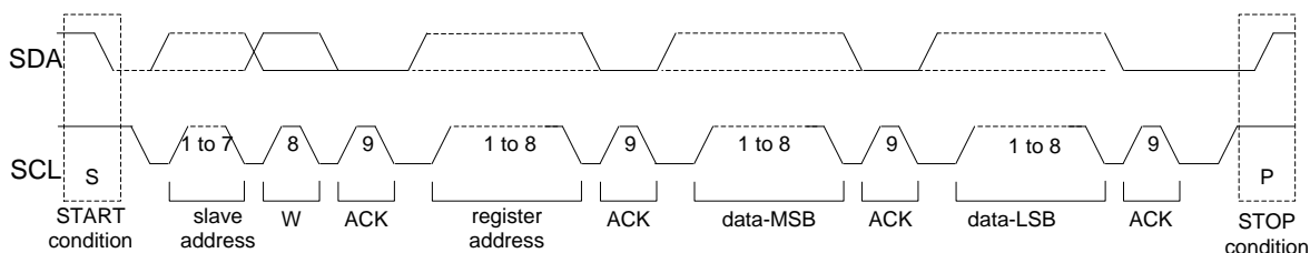
Figure 35. Write Sequence
