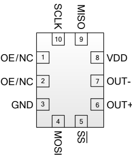
Figure 4. SPI Mode
