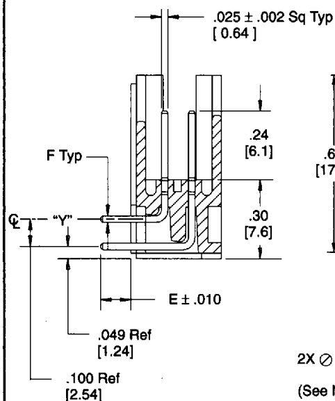
Section B-B (Right Angle)
