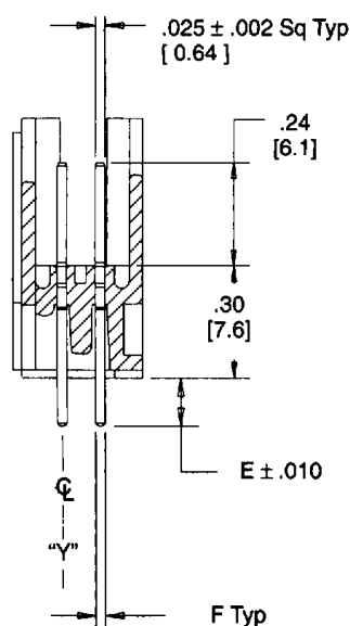
Section A-A (Straight)
