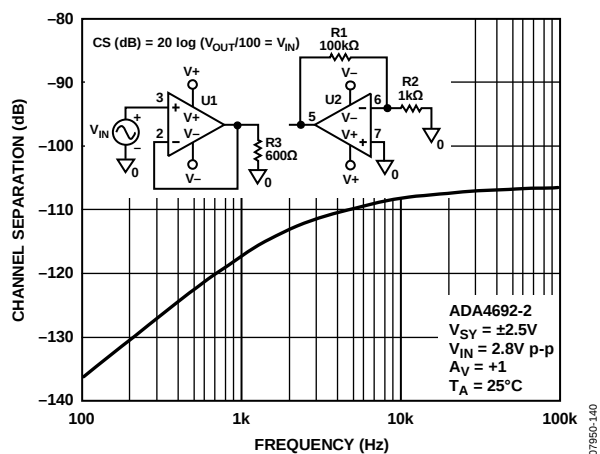
Figure 53. Channel Separation (CS) vs. Frequency
