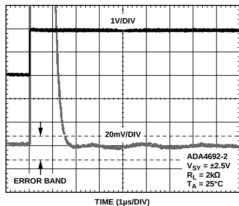
Figure 54. Positive Settling Time to 0.1%
