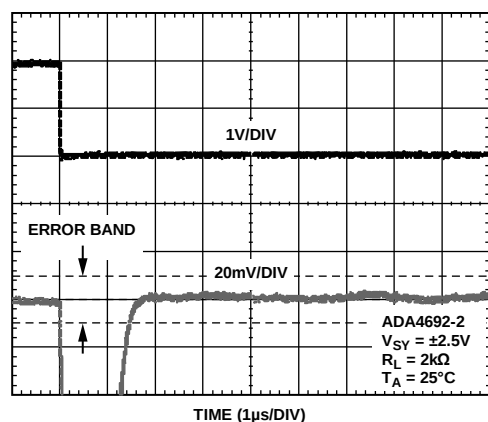
Figure 55. Negative Settling Time to 0.1%
