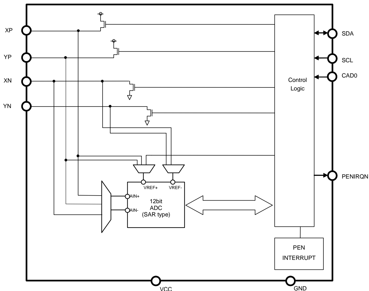
Block Diagram
