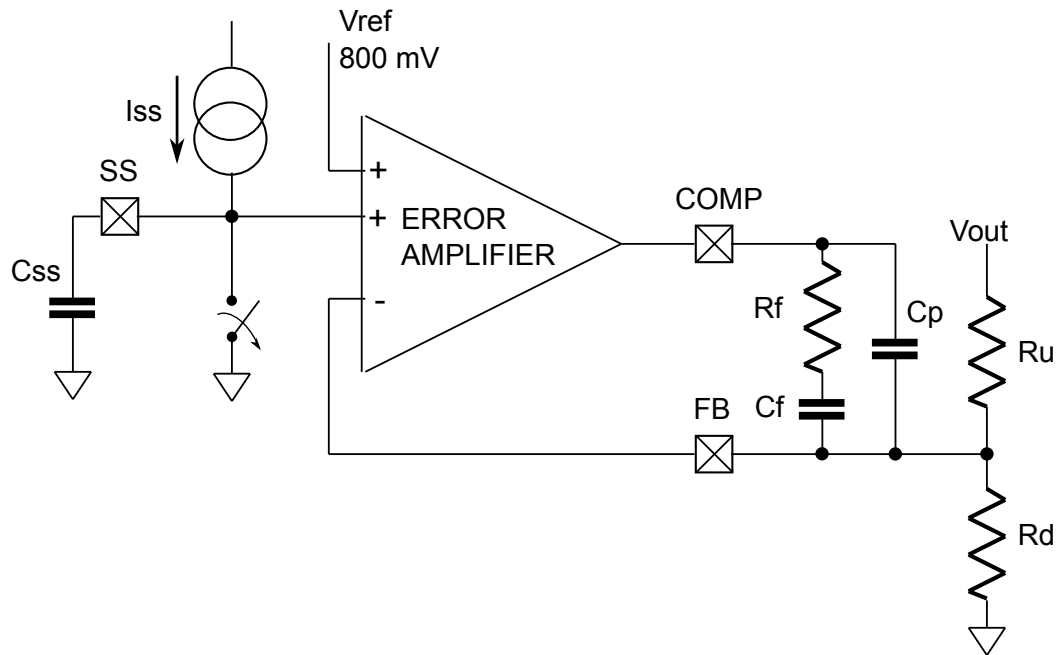
Figure 7. Soft-start
