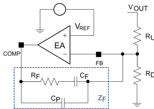
Figure 11. Type II compensation network
