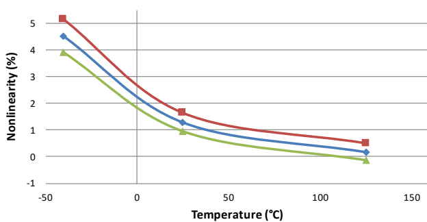
Linearity Error vs. Temperature
