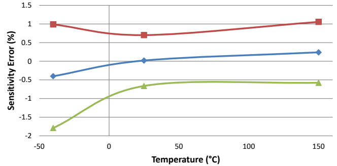
Sensitivity Error vs. Temperature
