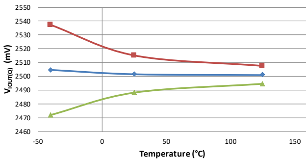
Zero Current Output Voltage vs. Temperature
