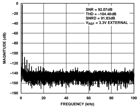
Figure 10. FFT, V_{REF} = 3.3 V External
