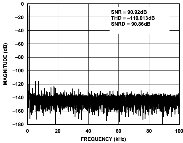
Figure 9. Fast Fourier Transform (FFT), V_{REF} = 2.5 V Internal
