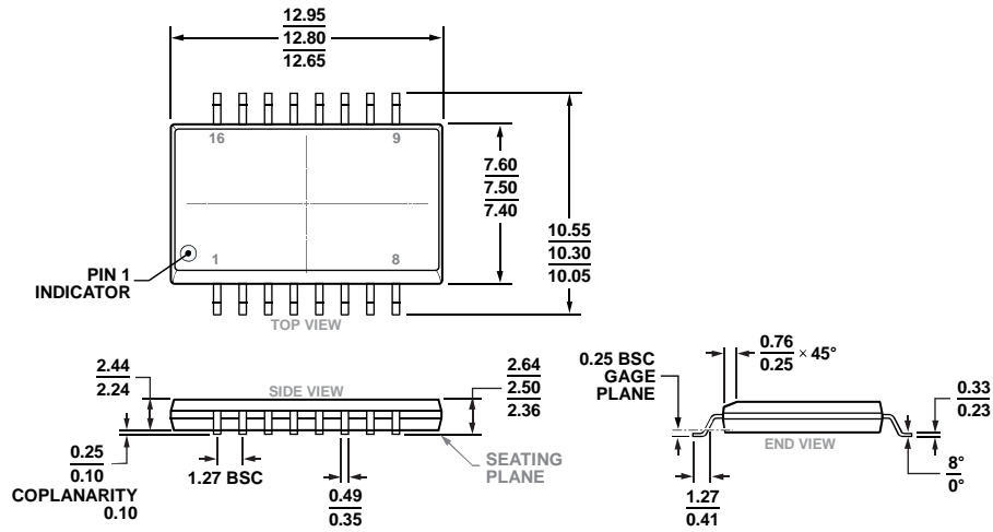
Figure 28. 16-Lead Standard Small Outline Package, with Increased Creepage [SOIC_IC] Wide Body (R1-16-2) Dimensions shown in millimeters
