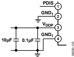
Figure 22. ADuM6028 V_{DDP} Bias and Bypass Components
