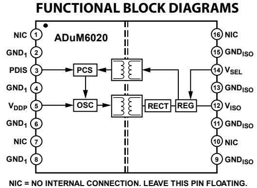
Figure 1. ADuM6020 Functional Block Diagram
