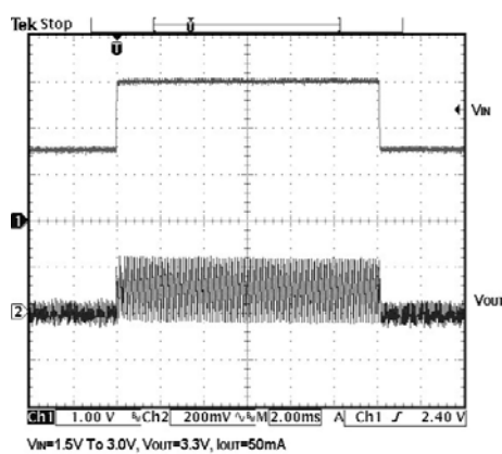
Line Transient
