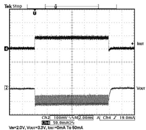
Load Transient
