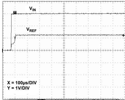
FIGURE 11. TURN-ON TIME
