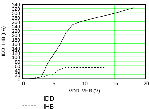
FIGURE 20. ISL2101A QUIESCENT CURRENT vs VOLTAGE
