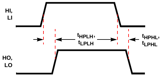
FIGURE 3. PROPAGATION DELAYS
