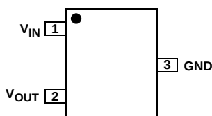
ISL21032 (3 LD SOT-23 TOP VIEW)
