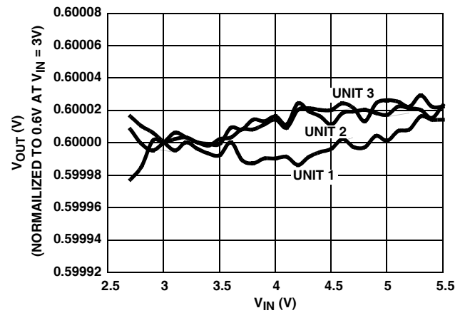
FIGURE 4. LINE REGULATION
