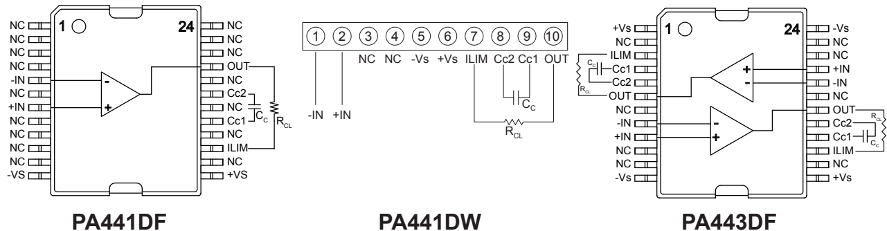
FIGURE 3. External Connections.
