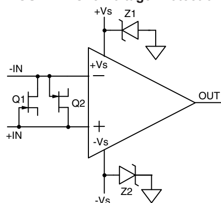
FIGURE 7. Overvoltage Protection
