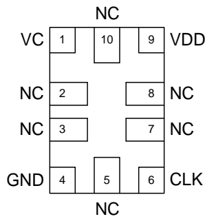
Figure 4. VCTCXO
