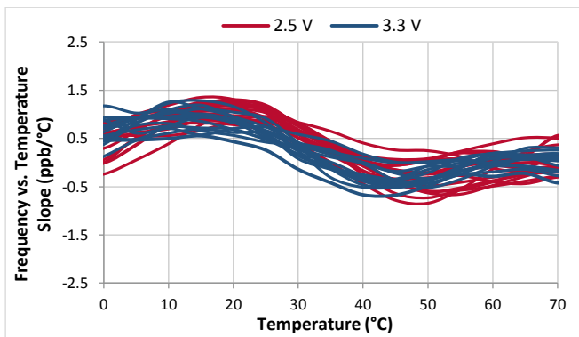
Figure 17. Freq. vs. Temp. Slope ( \Delta F/\Delta T )
