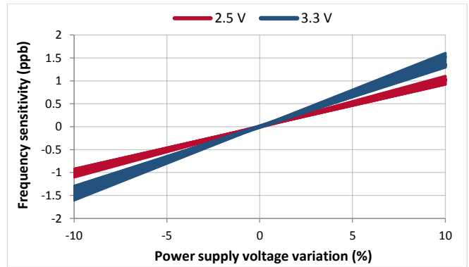
Figure 22. VDD sensitivity
