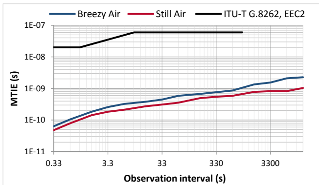
Figure 15. MTIE (0.1 Hz loop bandwidth)
