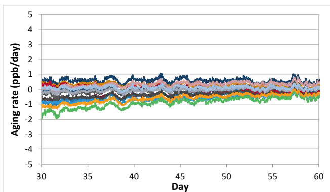
Figure 19. 1-day aging rate (to 62 days)
