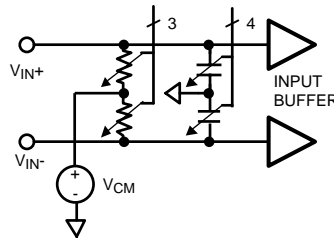
Figure 30. Simplified Input Differential Balance Correction Circuit
