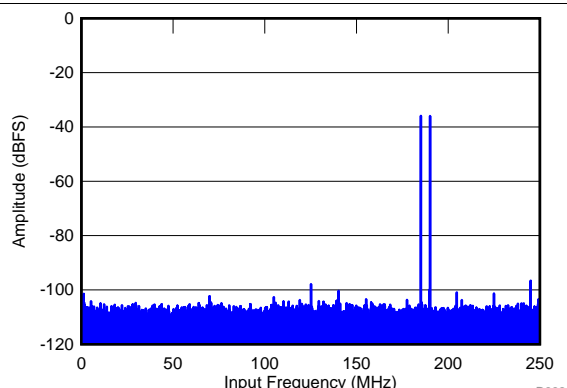
f_{\text{IN1}} = 185\text{ MHz} , f_{\text{IN2}} = 190\text{ MHz} , IMD = 103 dBFS, each tone at -36\text{ dBFS}
