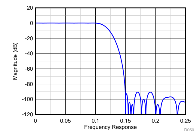
Figure 66. Frequency Response for Decimate-by-2, Low-Pass Filter (in Mode 6)
