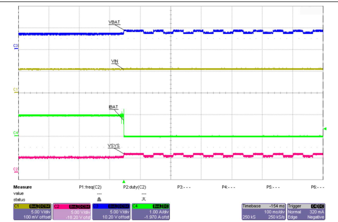
Figure 2. Battery Removal
