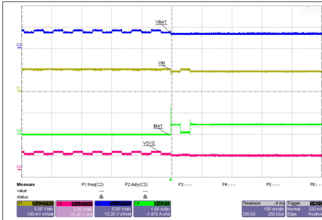
Figure 1. Battery Detection
