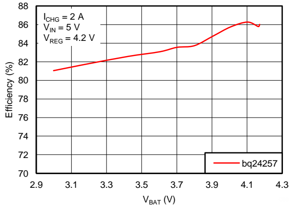
Figure 3. Efficiency vs. Battery Voltage
