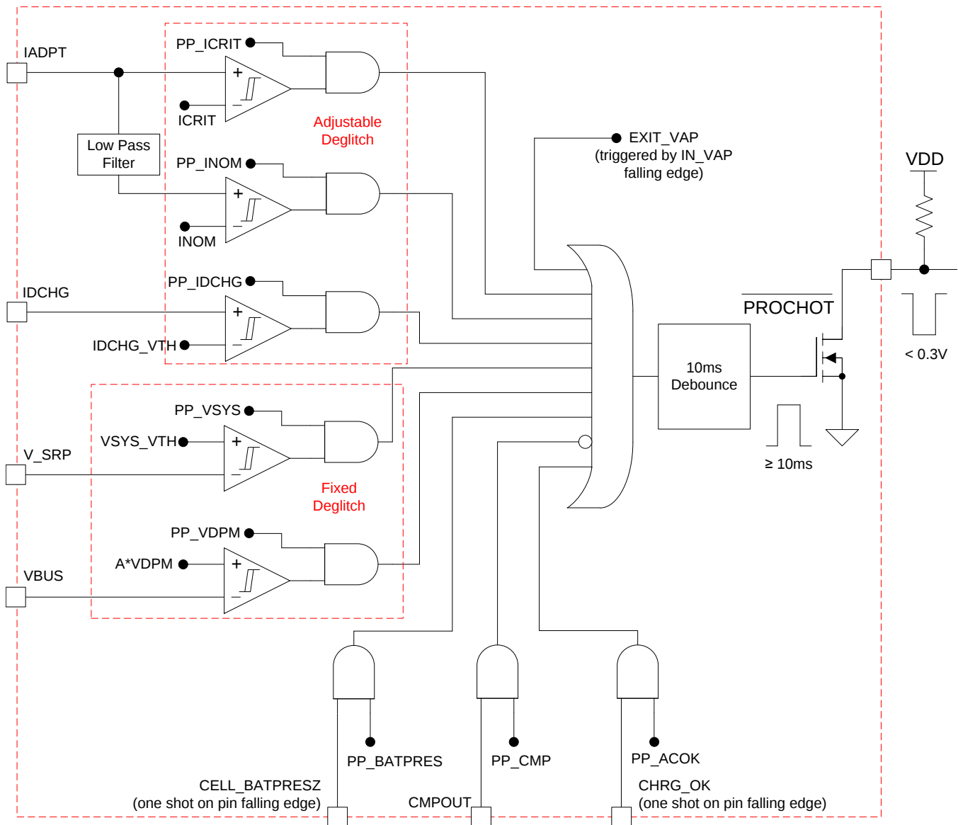
Figure 13. PROCHOT Profile
