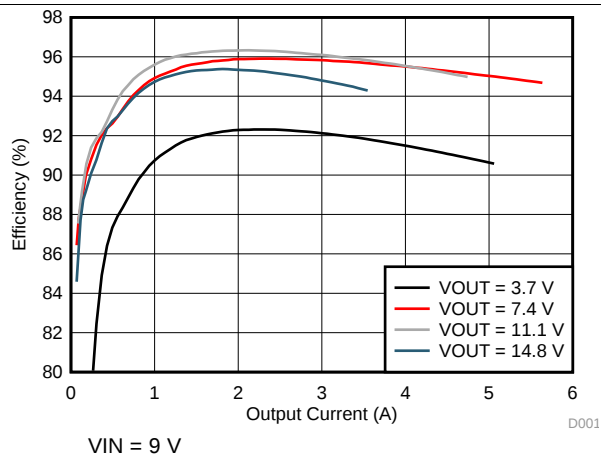
Figure 5. System Efficiency
