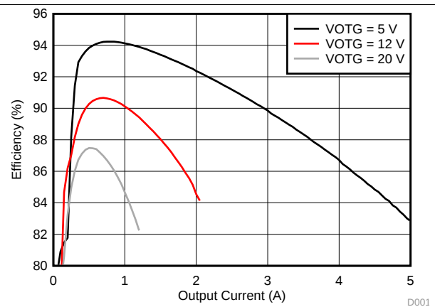
Figure 6. System Efficiency
