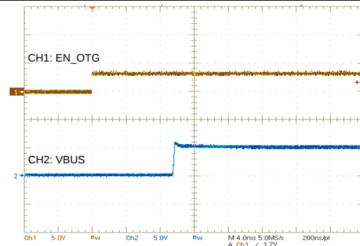
Figure 61. OTG Power Up from 8 V Battery
