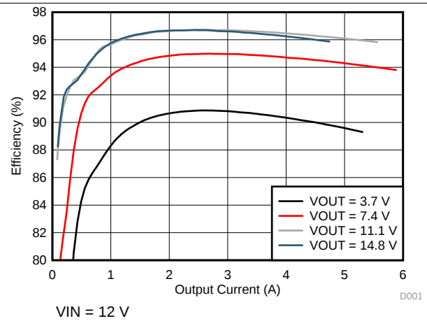
Figure 6. System Efficiency
