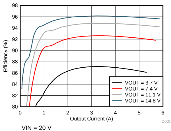
Figure 7. System Efficiency
