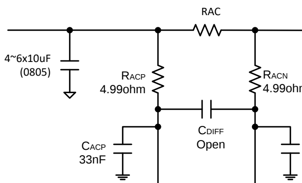
Figure 47. ACN-ACP Input Filter
