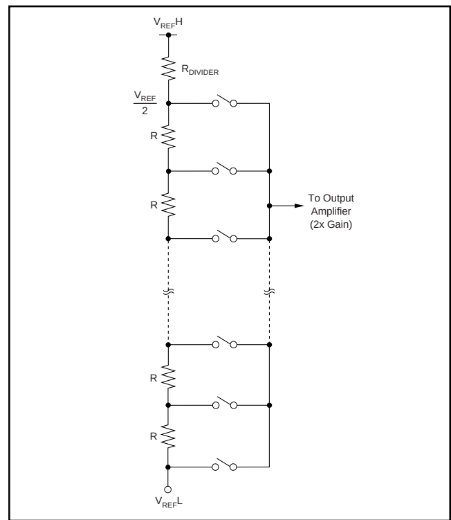
FIGURE 2. Resistor String.
