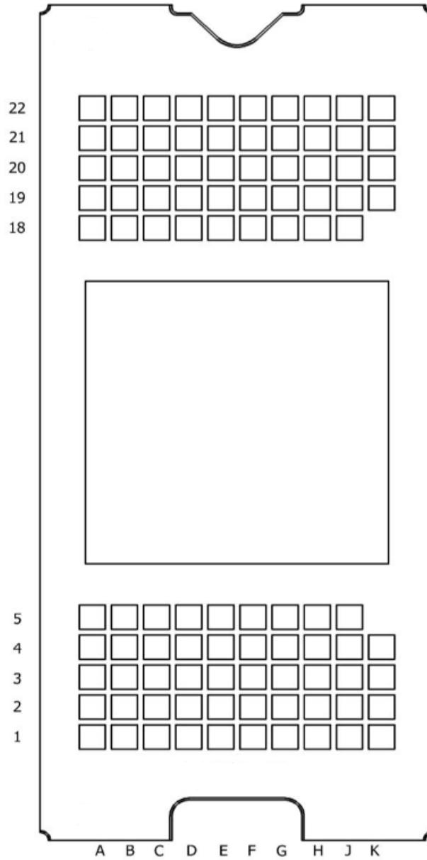
FQD Package LCCC (98) Bottom View
