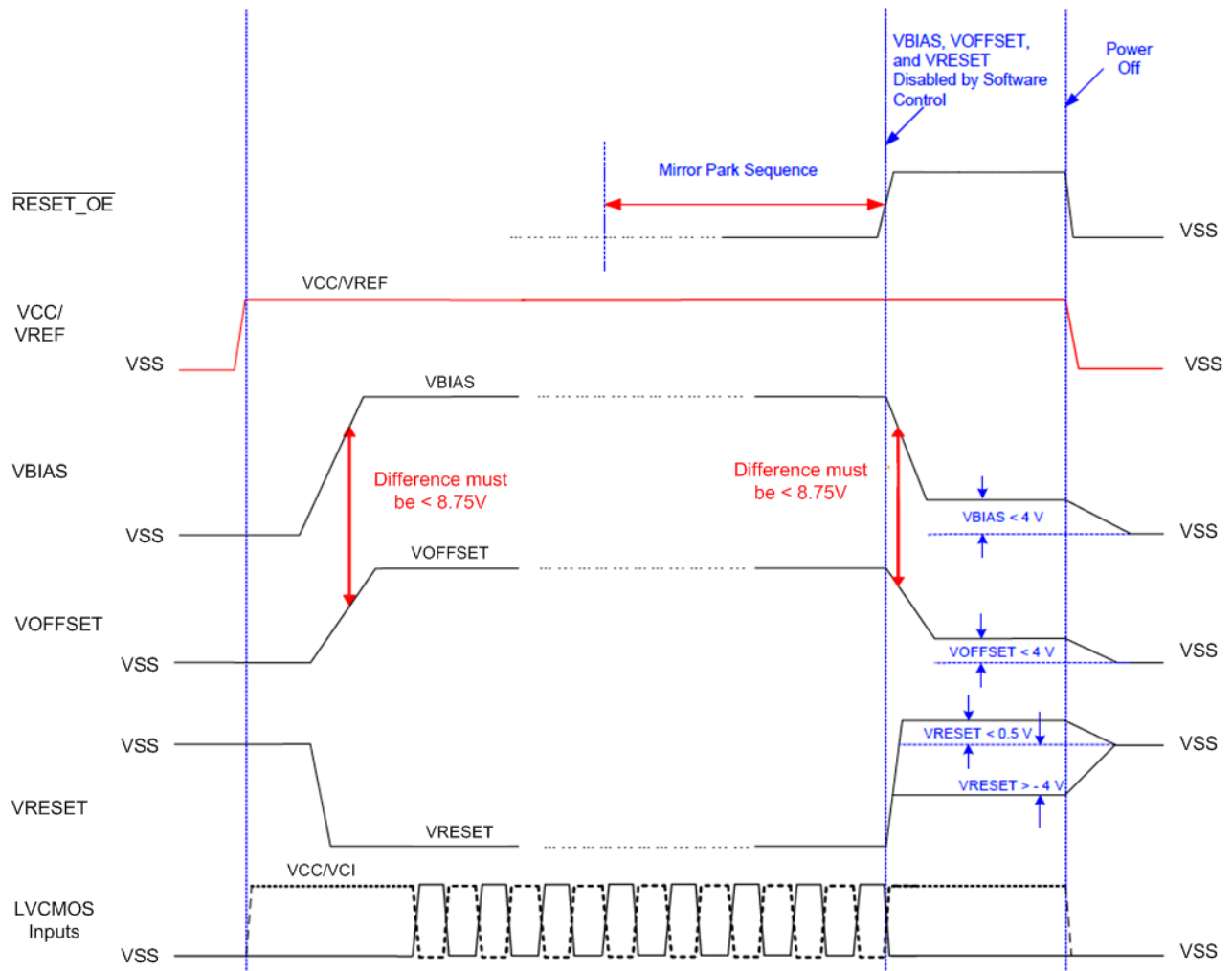
Figure 10. Power-Up and Power-Down Timing
