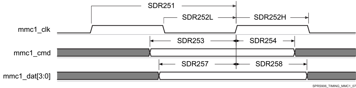
Figure 5-84. MMC/SD/SDIO in - High Speed SDR25 - Receiver Mode
