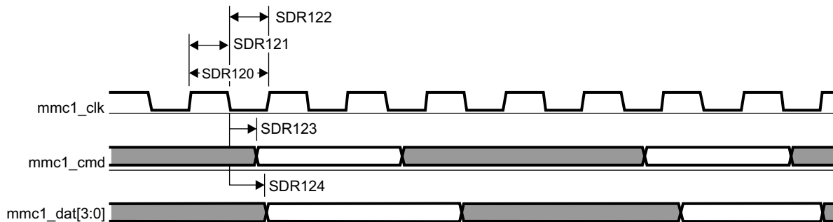
Figure 5-83. MMC/SD/SDIO in - High Speed SDR12 - Transmitter Mode
