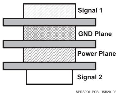
Figure 7-22. Four-Layer Board Stack-Up
