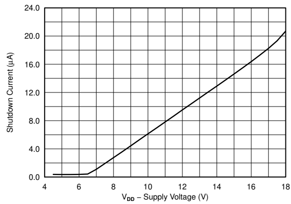
Figure 3. Shutdown Current vs VDD Voltage
