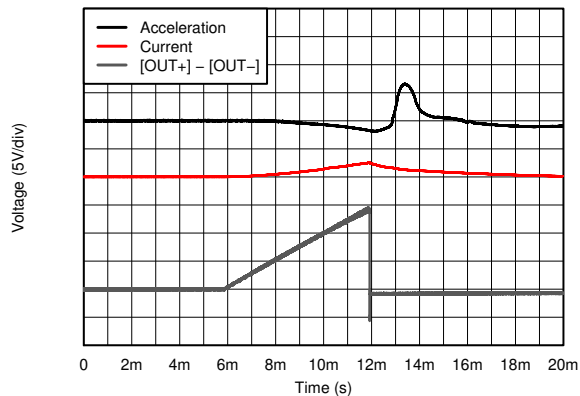
Figure 19. Voltage and Acceleration vs Time (Ramp Wave)
