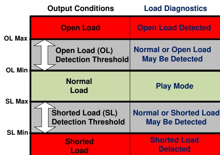
Figure 7. Load Diagnostic Reporting Thresholds
