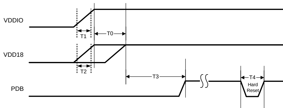
Figure 32. Power-Up Sequencing
