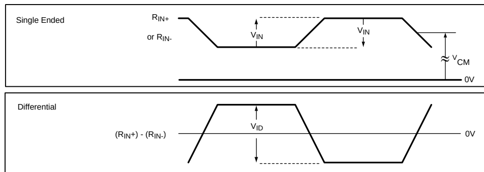
Figure 2. FPD-Link III Receiver V_{\text{ID}} , V_{\text{IN}} , V_{\text{CM}}
