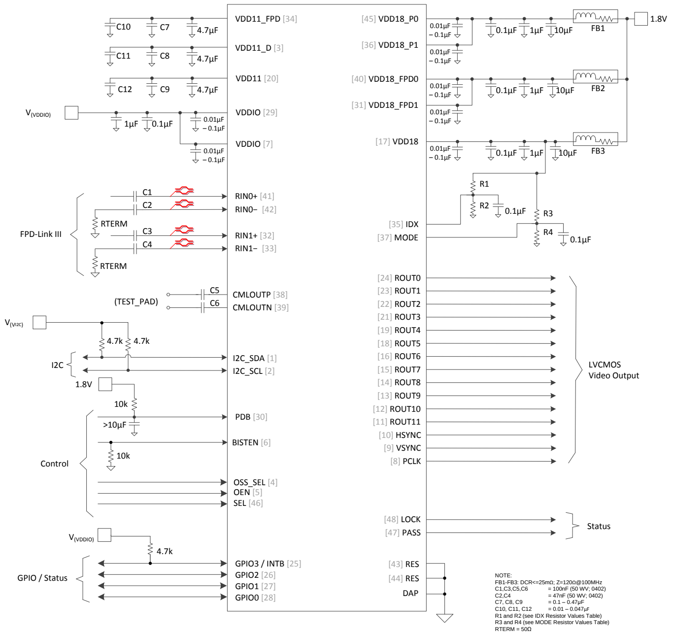
Figure 24. Typical Connection Diagram Coaxial
