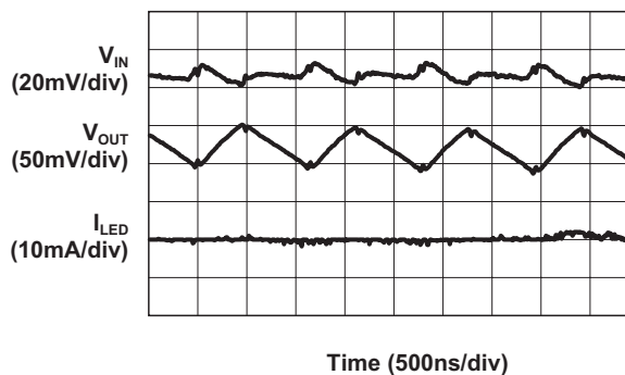
Load Characteristics ( V_{IN} = 2.7V ; 2X Mode; 20mA/ch Load)
