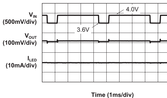
Line Response (20mA/ch Load)
