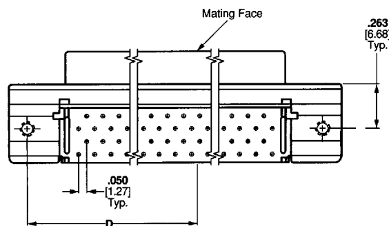
With Boardlocks
