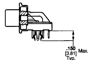
With Boardlocks
