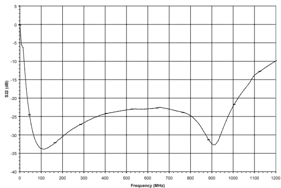
Figure 18: Output Return Loss vs. Frequency ( V_{DD} = +12\text{ V} , I_{DD} = 325\text{ mA} )
