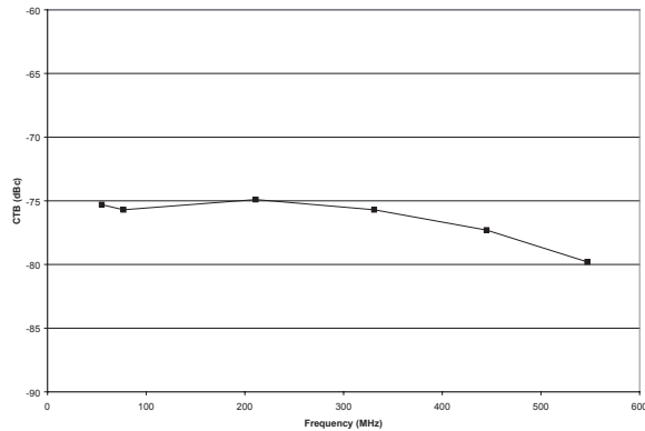
Figure 20: CTB vs. Frequency (V DD = +12 V, I DD = 325 mA, 79 Analog Channels, 15.6 dB Tilt, +49 dBmV output power at 1 GHz)
