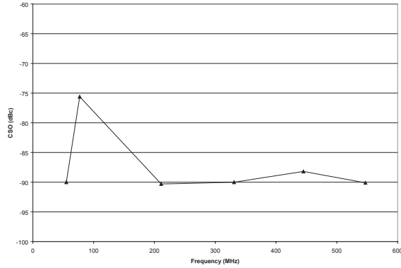
Figure 21: CSO vs. Frequency (V DD = +12 V, I DD = 325 mA, 79 Analog Channels, 15.6 dB Tilt, +49 dBmV output power at 1 GHz)
