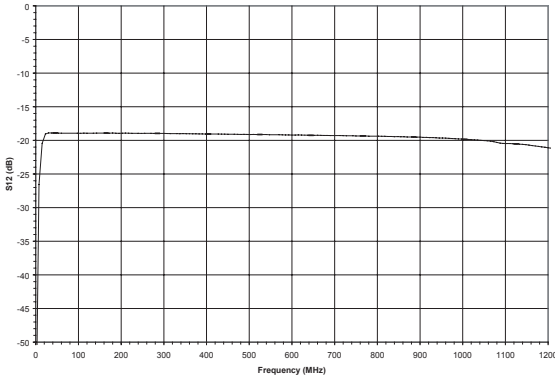
Figure 5: Reverse Isolation vs. Frequency (V DD = +12 V, I DD = 195 mA)
