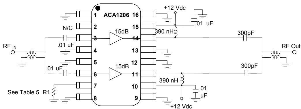
Figure 3: Test Circuit
