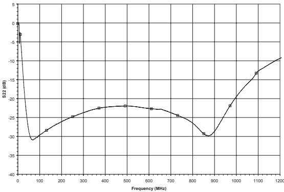
Figure 7: Output Return Loss vs. Frequency (V DD = +12 V, I DD = 195 mA)
