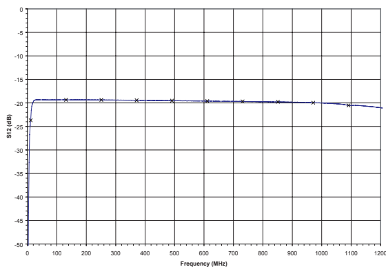
Figure 16: Reverse Isolation vs. Frequency ( V_{DD} = +12\text{ V} , I_{DD} = 325\text{ mA} )
