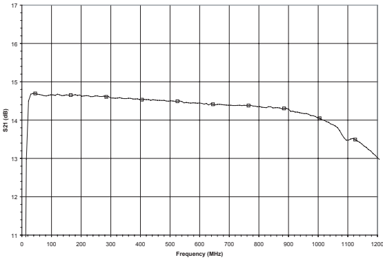
Figure 4: Gain vs. Frequency (V DD = +12 V, I DD = 195 mA)
