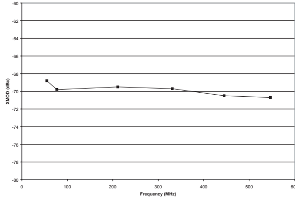
Figure 22: XMOD vs. Frequency (V DD = +12 V, I DD = 325 mA, 79 Analog Channels, 15.6 dB Tilt, +49 dBmV output power at 1 GHz)
