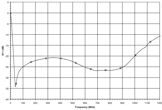
Figure 6: Input Return Loss vs. Frequency (V DD = +12 V, I DD = 195 mA)
