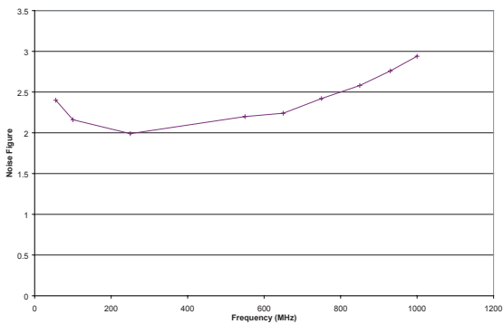
Figure 8: Noise Figure vs. Frequency (V DD = +12 V, I DD = 195 mA)
