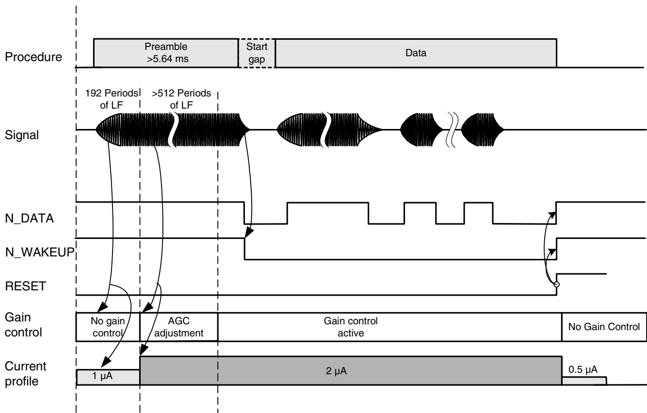
Figure 3. Communication Protocol
