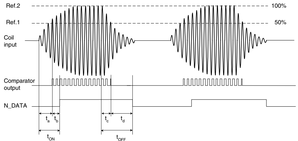
Figure 5. Output Timing
