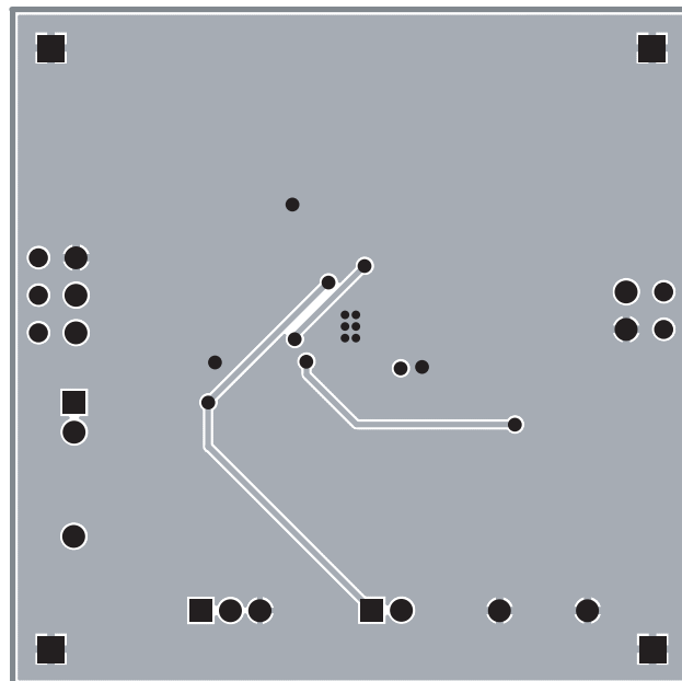
Figure 6: AAT3783 Evaluation Board Middle Layer.
