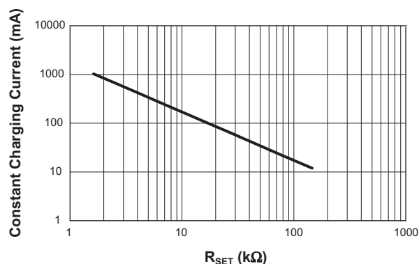
Figure 2: Constant Charging Current vs. Set Resistor Values.
