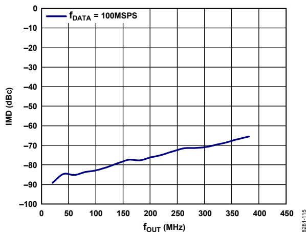
Figure 18. IMD vs. f_{OUT} , 8 \times Interpolation, f_{DATA} = 100 MSPS, Digital Scale = 0 dBFS, I_{FS} = 20 mA
