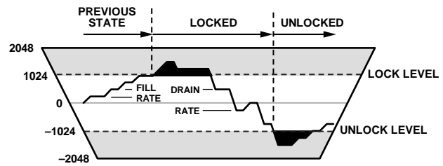
Figure 43. Lock Detector Diagram
