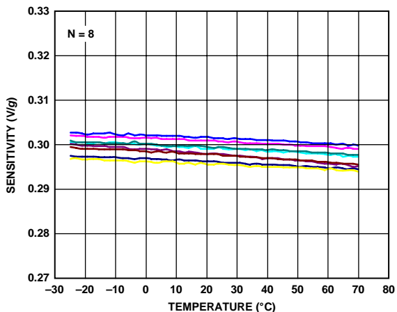
Figure 26. X-Axis Sensitivity vs. Temperature 8 Parts Soldered to PCB, V_S = 3V
